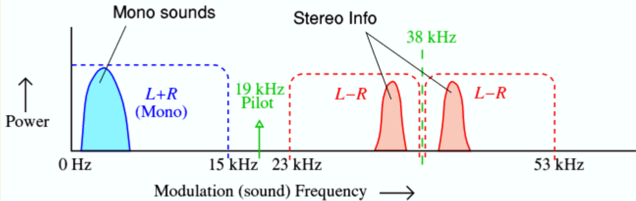
Fig 1 - FM Stereo Multiplex signal.
